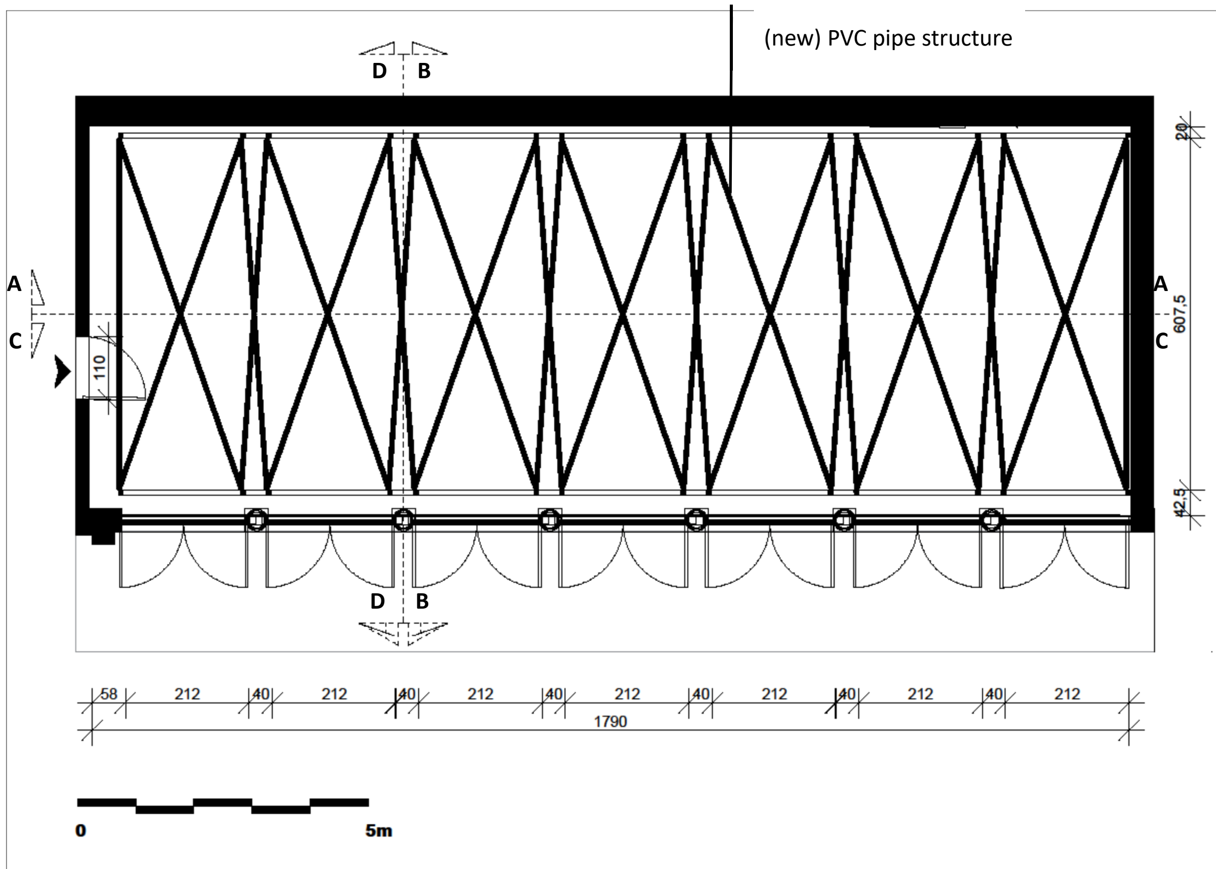
FLOOR PLAN / TUNNEL SCREEN - STRUCTURE / PVC PIPES
