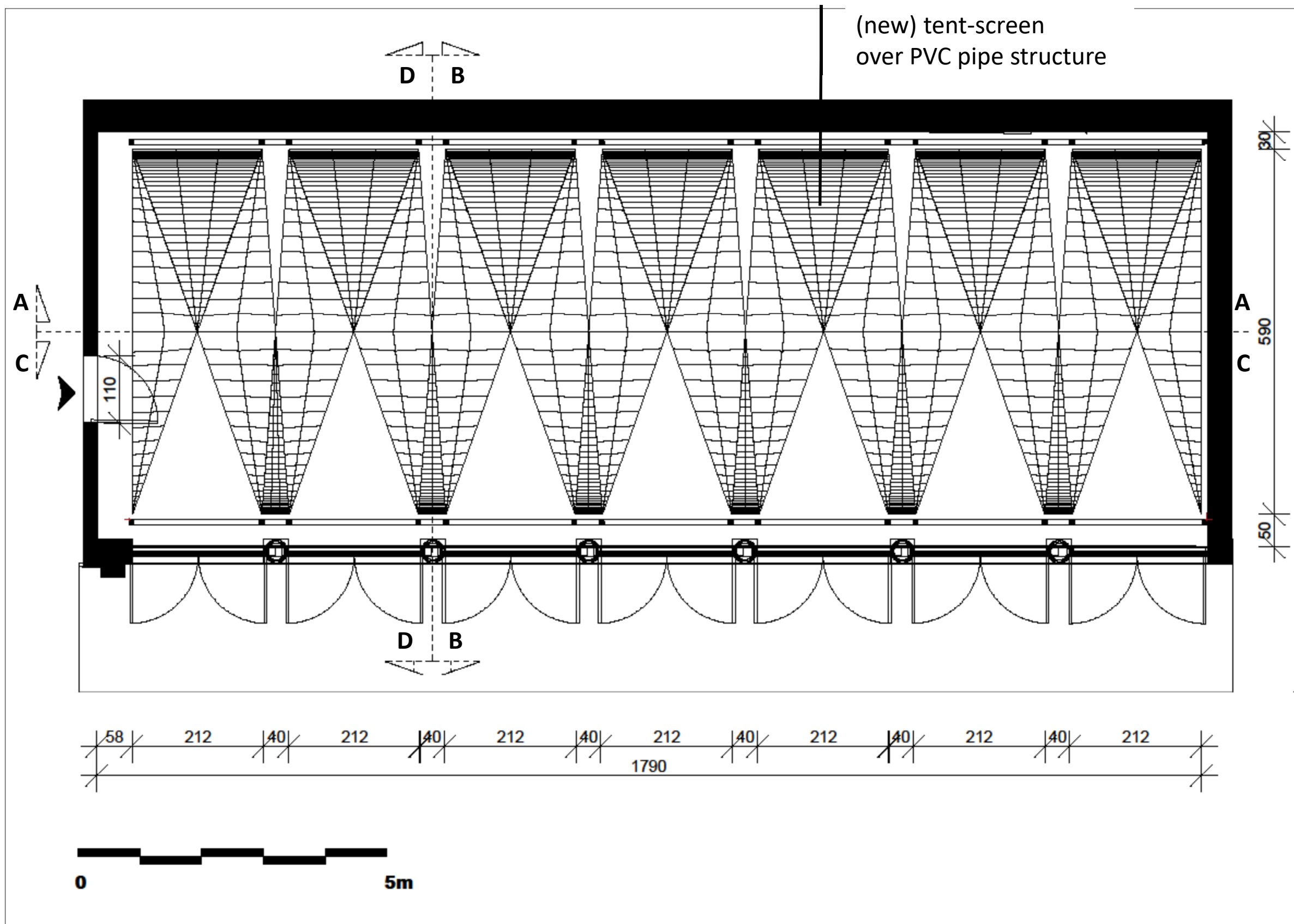
FLOOR PLAN / TUNNEL SCREEN - TENT
